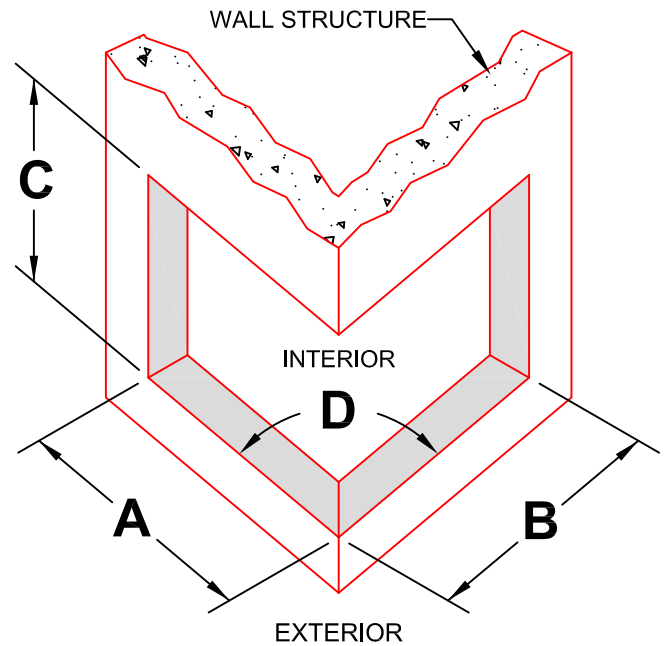
ISOMETRIC VIEW LESS THAN 90° OUTSIDE CORNER STRUCTURE
