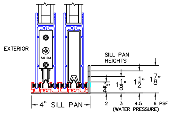
SERIES 3070 NO RISER (STANDARD)
