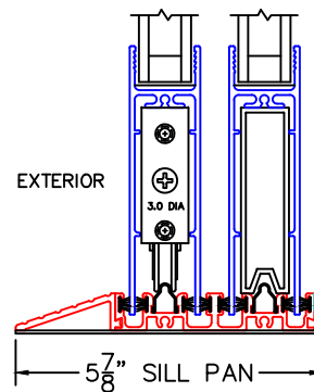
SERIES 3070 EXTERIOR RISER (OPTIONAL)
