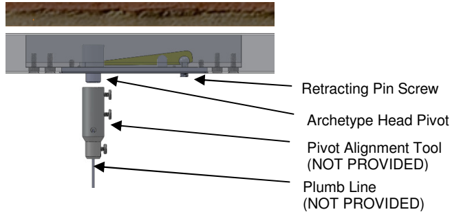
Figure 13: In-line Verification
