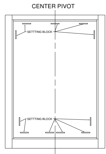
Figure 22: Center Pivot Location Setting Blocks
