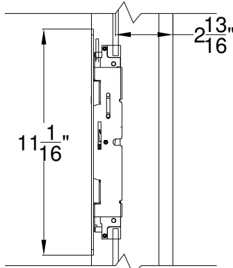
Figure B3: Inactive Panel Shoot-bolts
