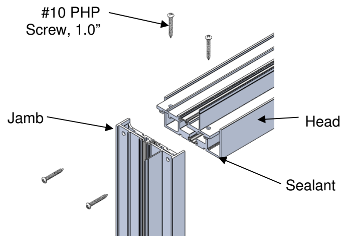
Figure 5: Frame Assembly
