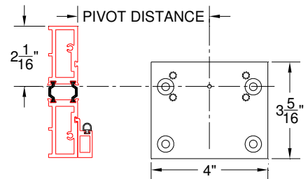
Exterior Figure 14: Archetype Floor Pivot Positioning
