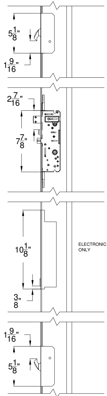
Figure A2: 5 Point Latch / Electronic Latch
