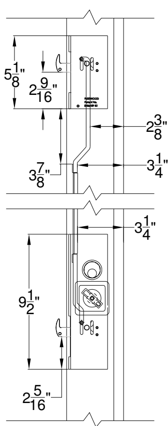
Figure A1: Archetype Latch and Secondary Latch
