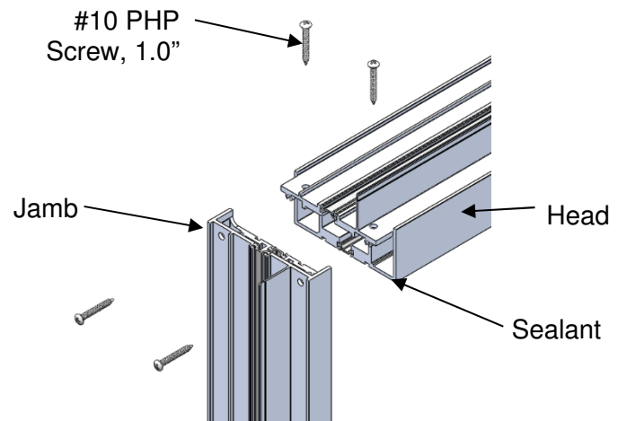
Figure 5: Frame Assembly
