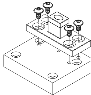
Figure 12: Archetype Floor Pivot Assembly
