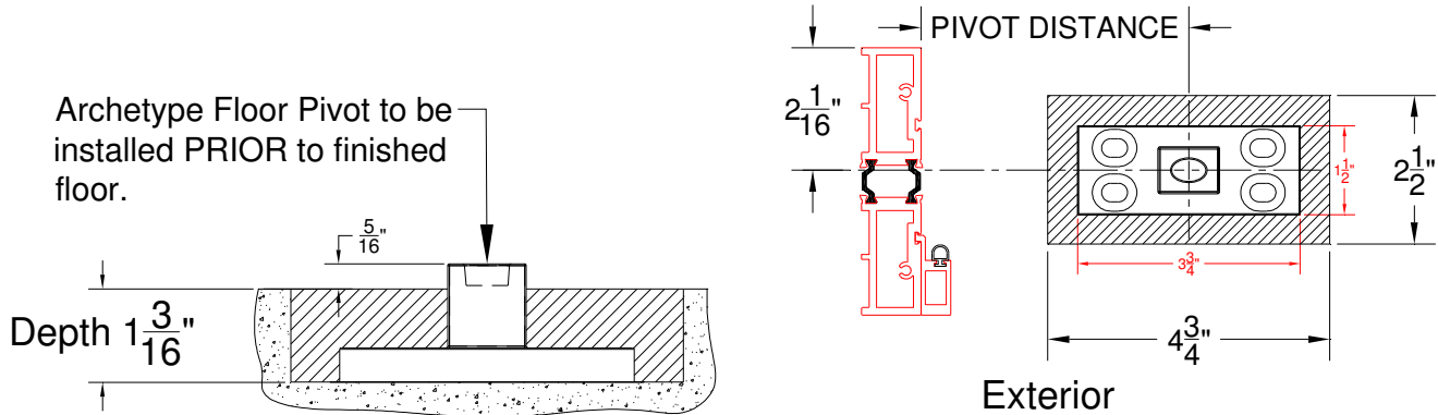
Figure C1: AFP-R Block Out and Positioning
