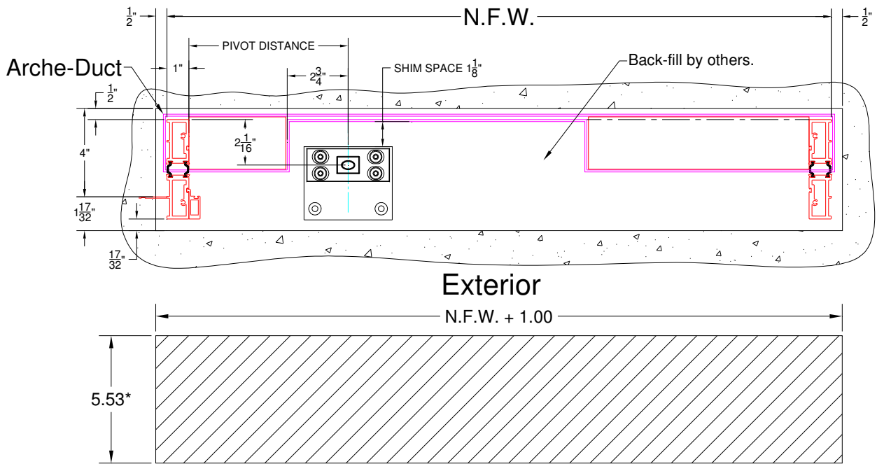
Figure 1: Arche-Duct Block Out (Top View)
