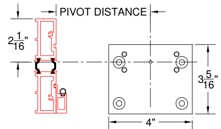
Exterior Figure 10: Archetype Floor Pivot Positioning
