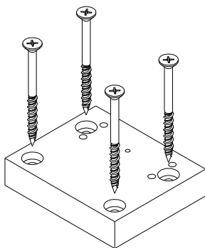
Figure 11: Securing the Archetype Floor Pivot
