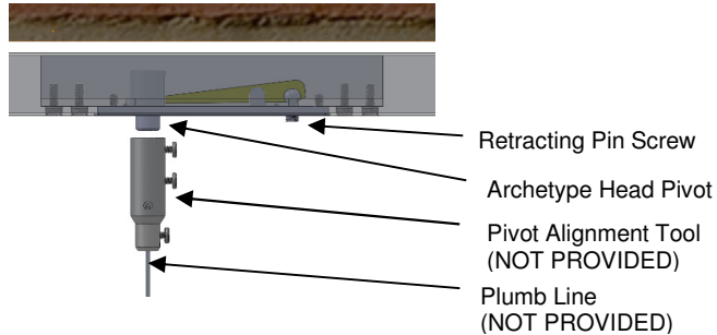
Figure 9: In-line Verification
