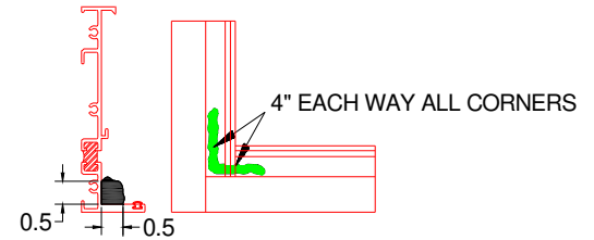
Figure 14: Sealant Location and Sizes
