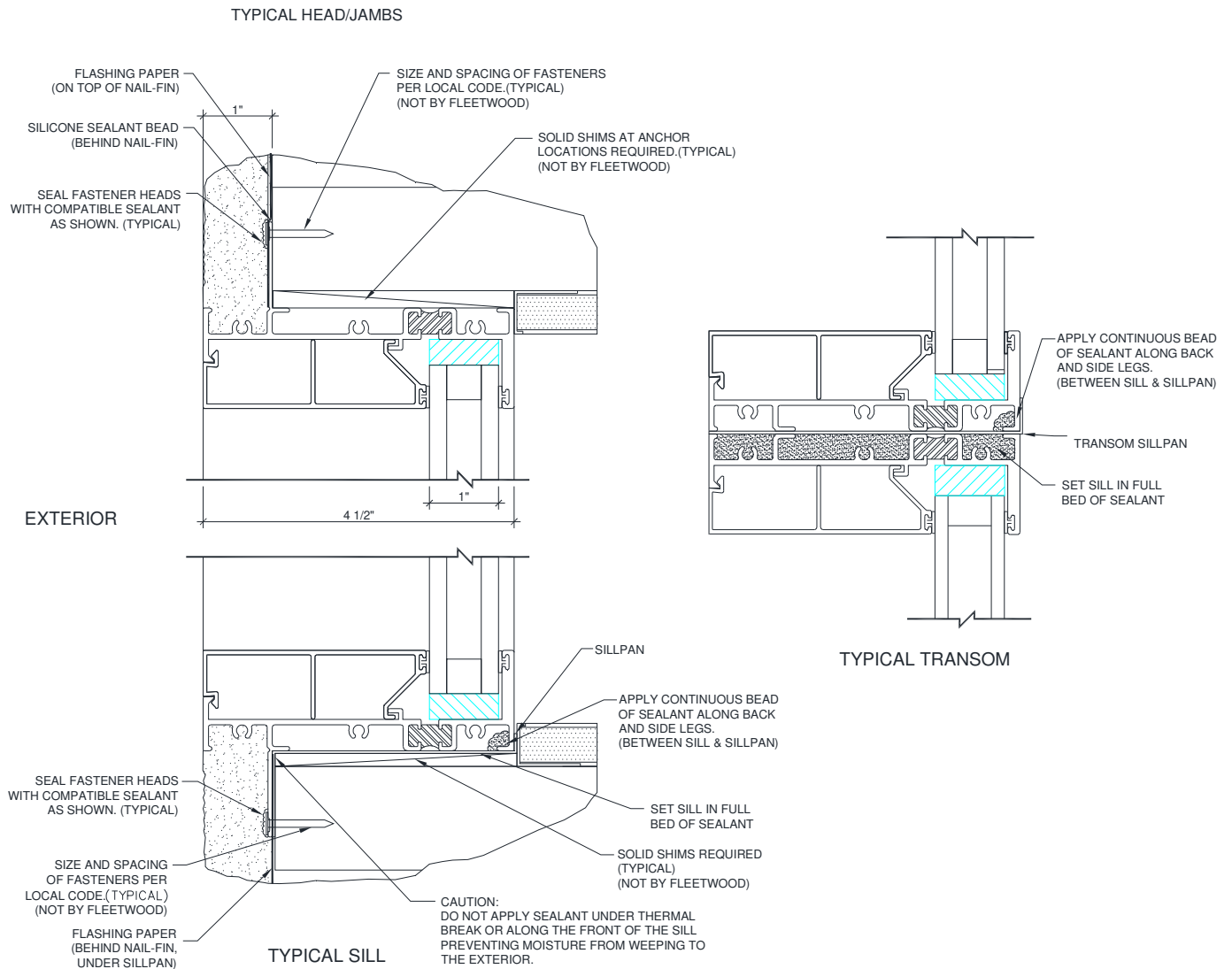
Figure 10: Typical Nail-fin with Sealant Shown (Exterior Glazed)
