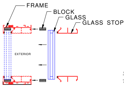
Figure 13: Setting Block Locations
