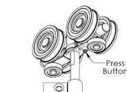
Figure A5: Intermediate Hanger Adjustment
