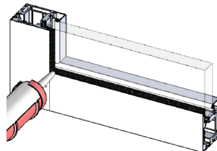
Figure 34: Inside glazed cap bead
