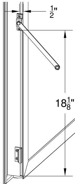
Figure 4: Limit Arm Location (LH Window Vent Illustrated)
