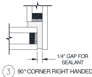
Figure 19: Dual Glaze Butt Glazing Options
