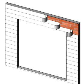
Figure 23: Building Flashing
