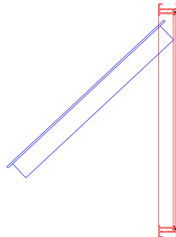
Figure C2: Vent In Open Position (Block Frame Shown)
