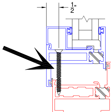
Figure C1: Vent Fastener Location (Block Frame Sill Shown)
