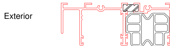
Figure 20: Sill Track Removal
