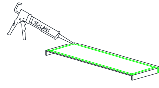
Figure 11: Seal underside of Sillpan
