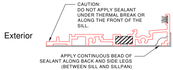
Figure 14: Attached Sill
