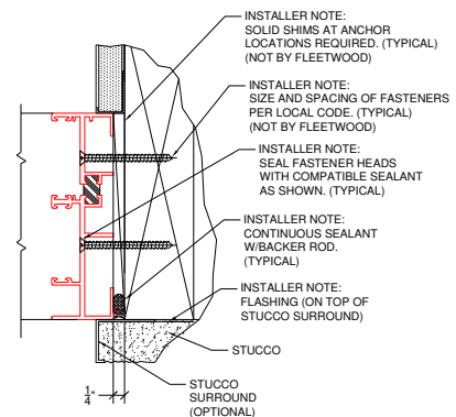
Figure 16: Block Frame Anchoring
