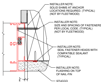
Figure 15: Nail-fin Anchoring
