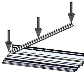
Figure 18: Sill Track Installation
