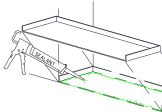
Figure 12: Set Pan in full bed of sealant
