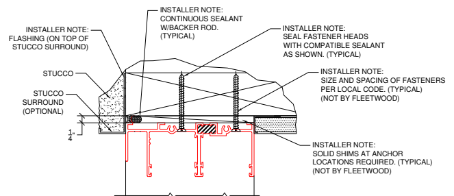
Figure 14: Attached Sill
