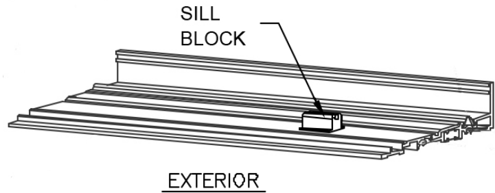
Figure 24: Attached Sill Block
