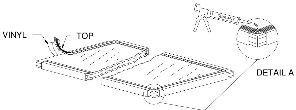
Figure 1: Glazing Vinyl Application
