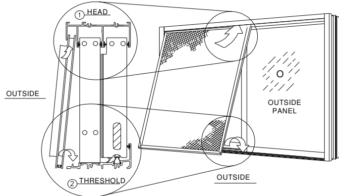
Figure 27: Screen Installation
