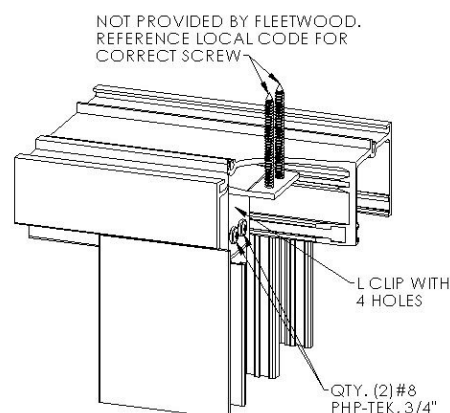
Figure 23: "L" Bracket at False Jamb / Frame Head
