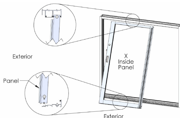
Figure 13: “X” Panel Installation
