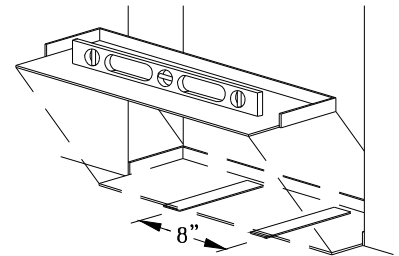
Figure 6: Leveling Sillpan
