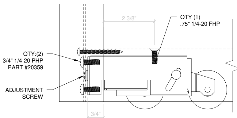
Figure 2: Roller Adjustment
