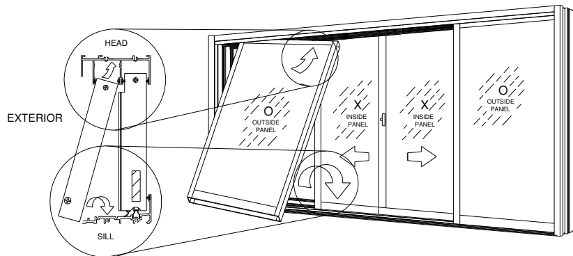
Figure 32: Sill Track Removal
