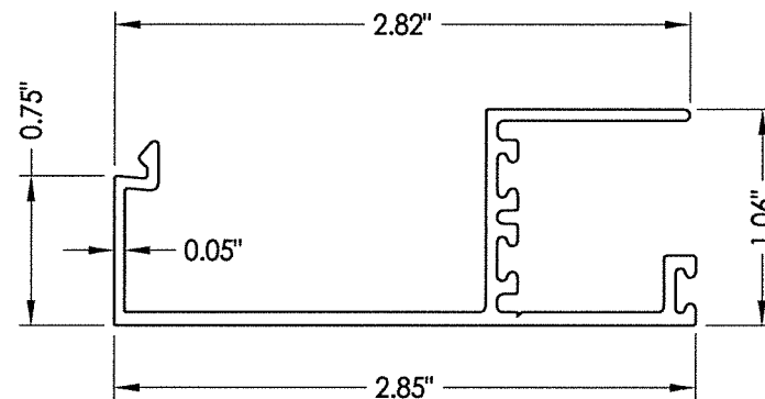
3 GLASS STOP 1-1/4"
