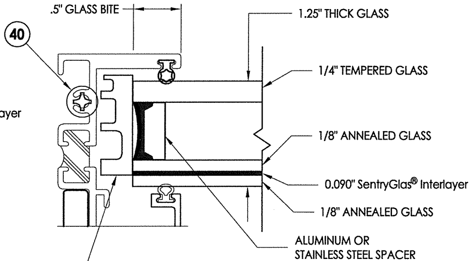
G5 GLAZING DETAIL
