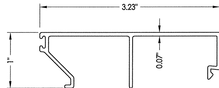
18 GLASS STOP 1"
