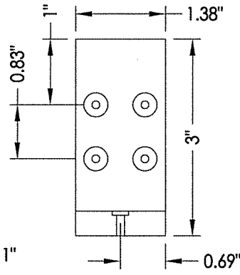
32 L BRACKET
