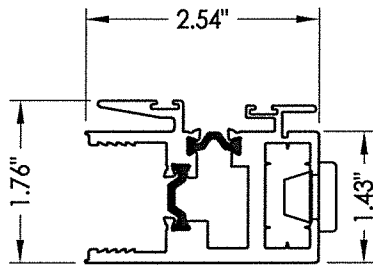
10 FIXED INTERLOCK
