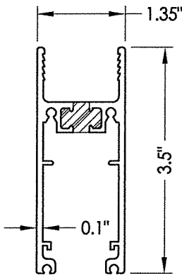
7 SLIDING BOTTOM RAIL
