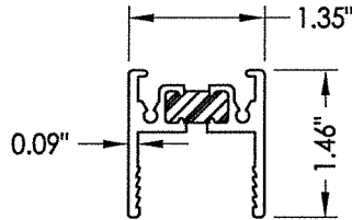
6 TOP RAIL
