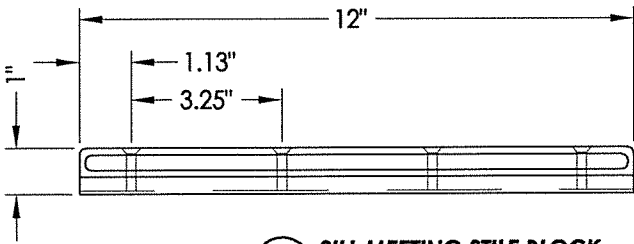
35 SILL MEETING STILE BLOCK
