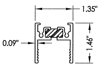
6 TOP RAIL
