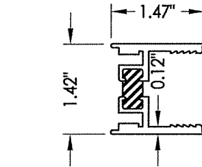
5 FIXED STILE
