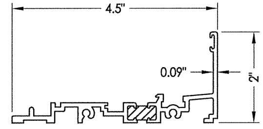
2 SILL
