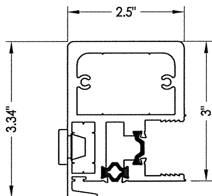
2 SILL
