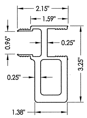
13 WINDLOAD ADAPTER
