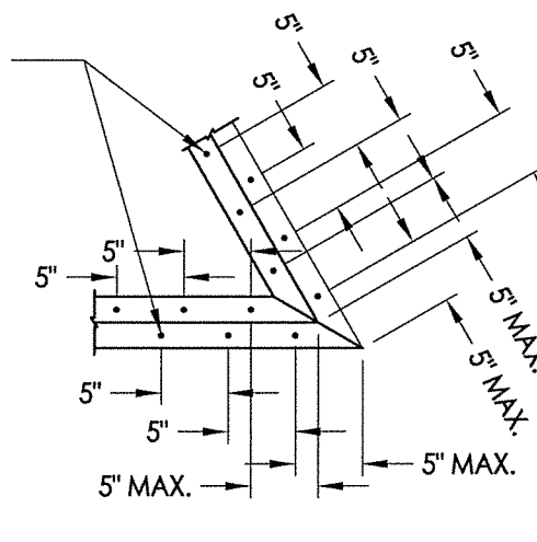
DETAIL 2 60° Corner
