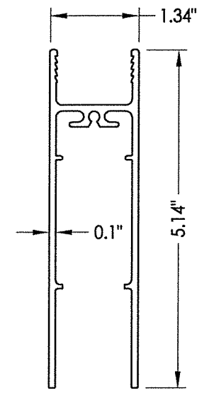
7 BOTTOM RAIL
