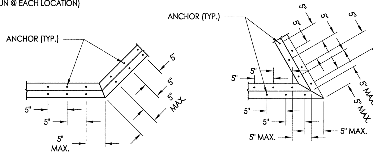
DETAIL 1 135° Corner
