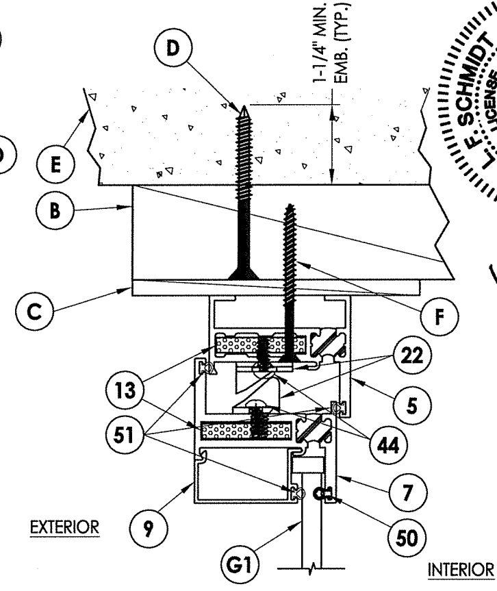
5 2 VERTICAL CROSS SECTION Shown w/ 2X Buck Construction
