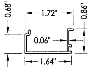
9 GLASS STOP 1/4"
