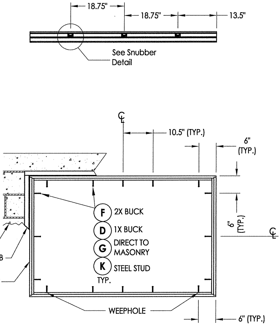
FRAME MOUNT ANCHORING 65" X 42" Max Size
