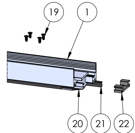
DETAIL E
