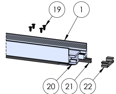
DETAIL E
