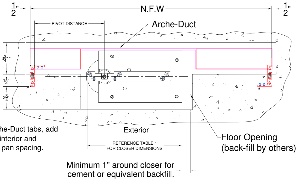
Figure A1: Closer Arche-Duct Opening (weatherseals removed for clarity only)
