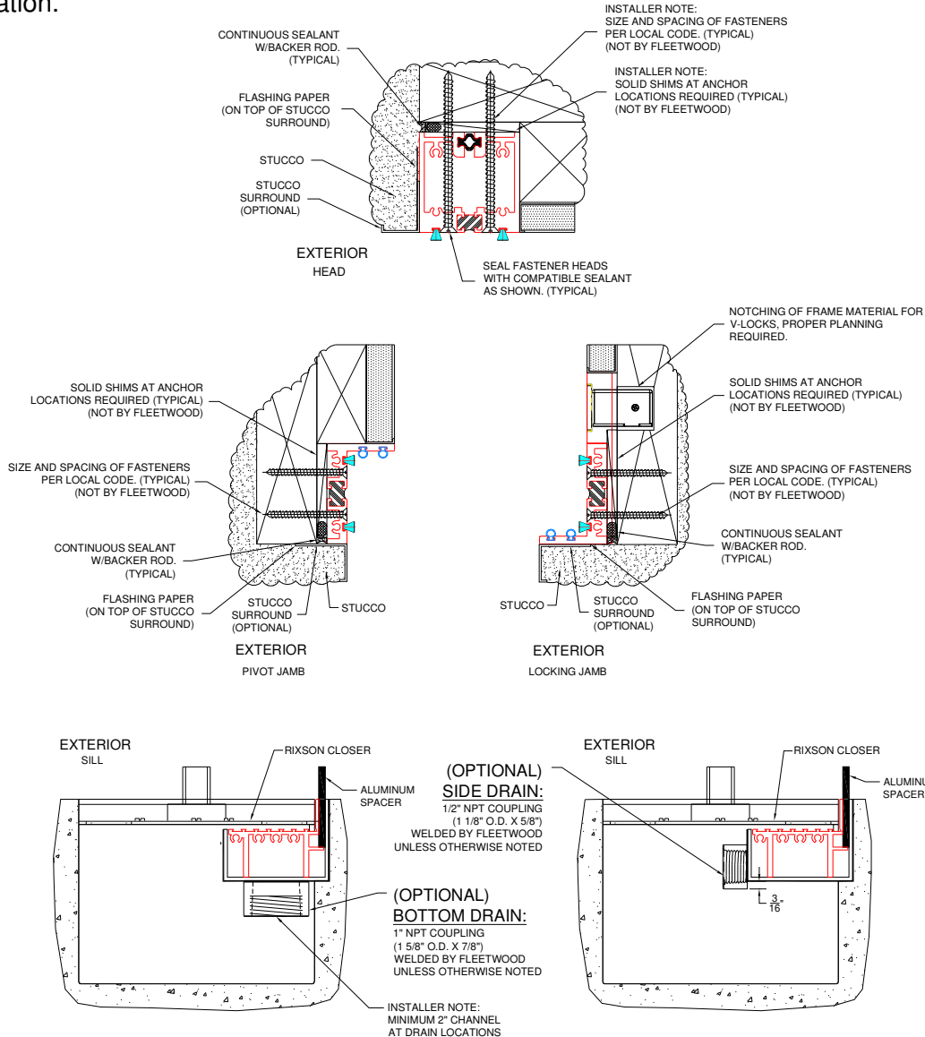
Figure 6: Closer Block Frame Installation
