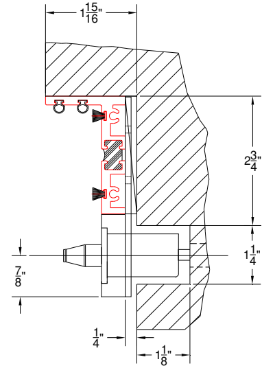
Figure D2: Plan View V-Lock Knockout
