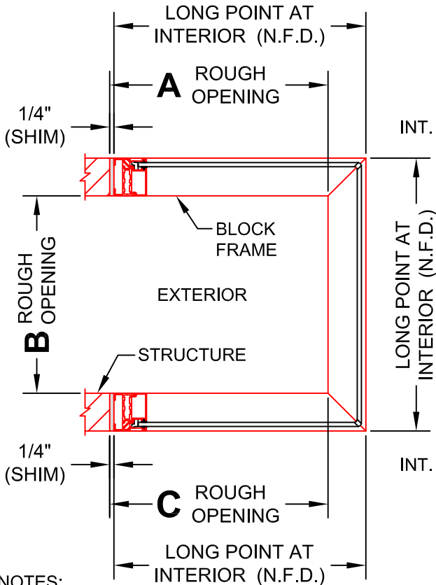
PLAN VIEW SERIES 350-T SHOWN
