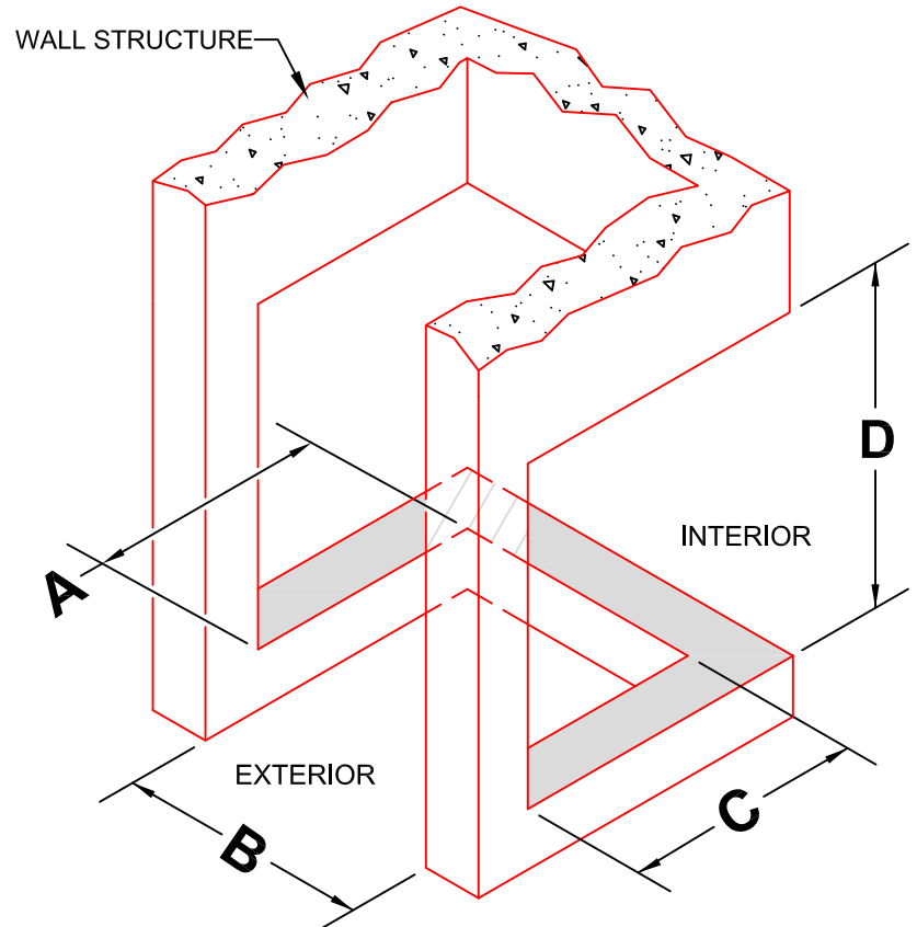
ISOMETRIC VIEW 90° INSIDE U-SHAPE STRUCTURE
