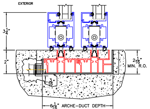
3A 1/2" SIDE DRAIN TO EXTERIOR (OPT-E2)
