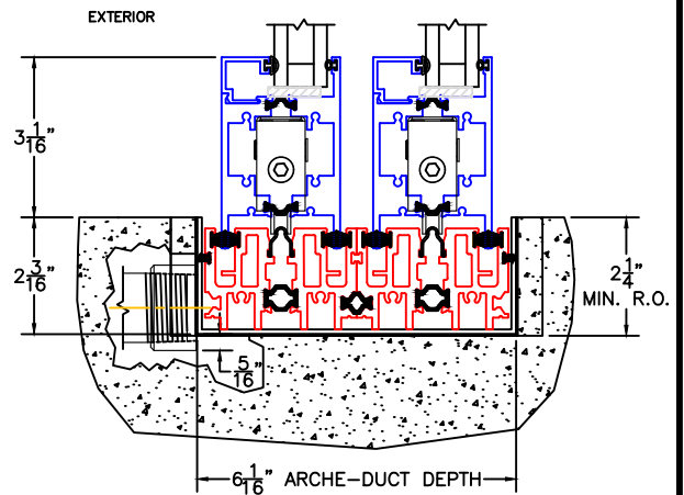
2A 1" SIDE DRAIN TO EXTERIOR (OPT-E1)
