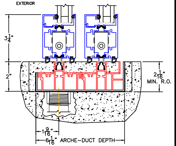
1A 1" BOTTOM DRAIN TO EXTERIOR (OPT-B)
