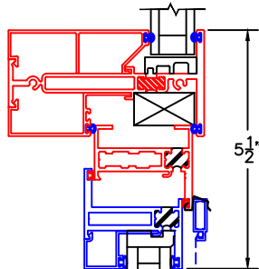
① HORIZONTAL TDL
