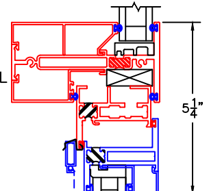
⑤ HORIZONTAL TDL
