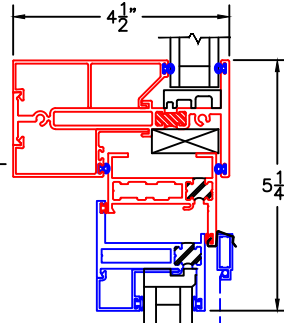
③ HORIZONTAL TDL
