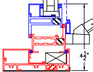
② BLOCK SILL W/ SILL PAN
