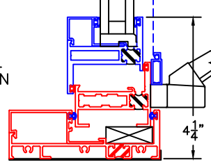
⑥ BLOCK SILL W/ SILL PAN
