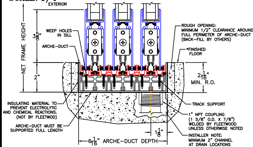
1 1" BOTTOM DRAIN TO INTERIOR (OPT-A)
