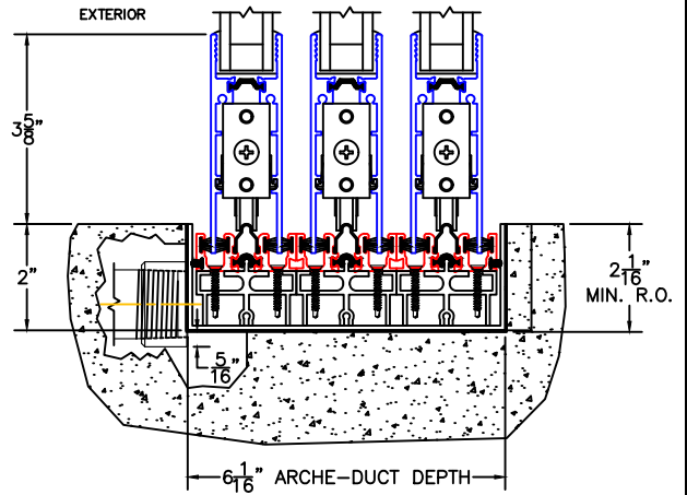
2A 1" SIDE DRAIN TO EXTERIOR (OPT-E1)
