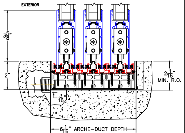
3A 1/2" SIDE DRAIN TO EXTERIOR (OPT-E2)
