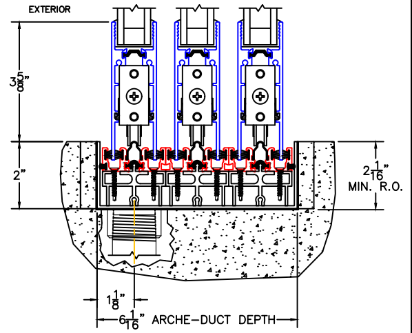
1A 1" BOTTOM DRAIN TO EXTERIOR (OPT-B)
