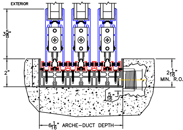
2 1" SIDE DRAIN TO INTERIOR (OPT-D1)
