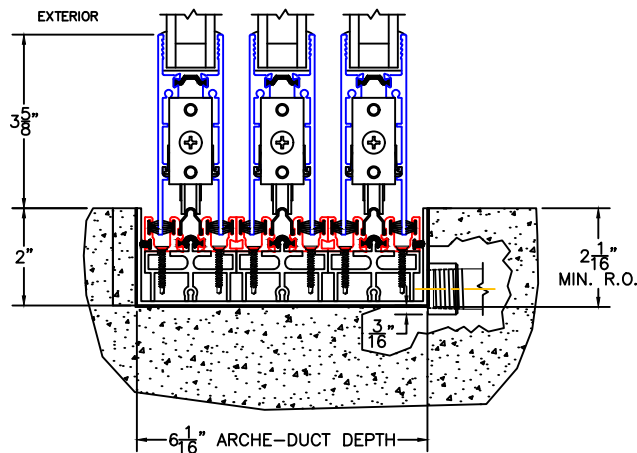
3 1/2" SIDE DRAIN TO INTERIOR (OPT-D2)
