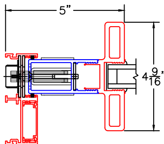
ARCHETYPE NARROW LOCK STILE WITH HP2 ADAPTER
