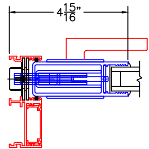
ARCHETYPE LOCK STILE WITH LEVER
