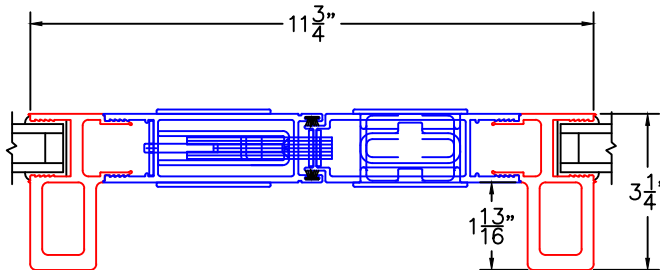
ARCHETYPE MEETING STILES WITH HP1 ADAPTERS
