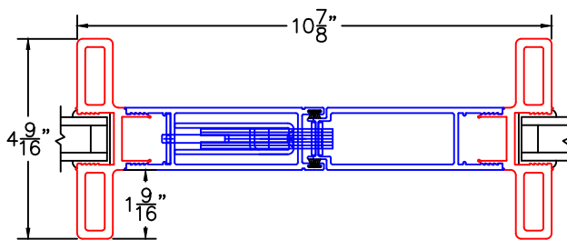
ARCHETYPE MEETING STILES WITH HP2 ADAPTERS
