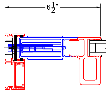
ARCHETYPE LOCK STILE WITH HP1 ADAPTER
