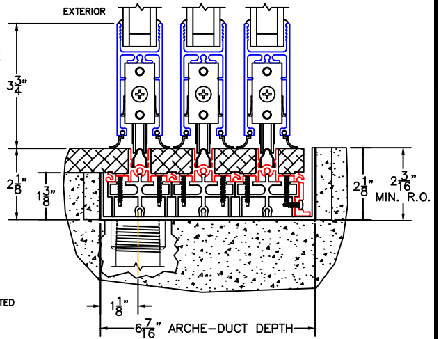
1A 1" BOTTOM DRAIN TO EXTERIOR (OPT-B)
