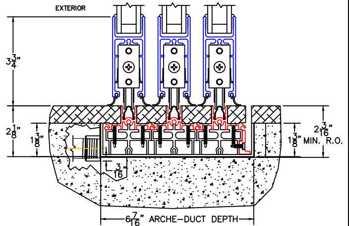
2A 1/2" SIDE DRAIN TO EXTERIOR (OPT-E2)
