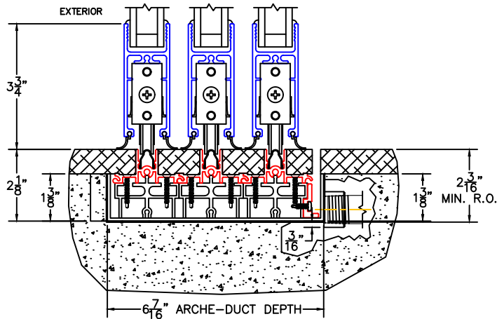
2 1/2" SIDE DRAIN TO INTERIOR (OPT-D2)
