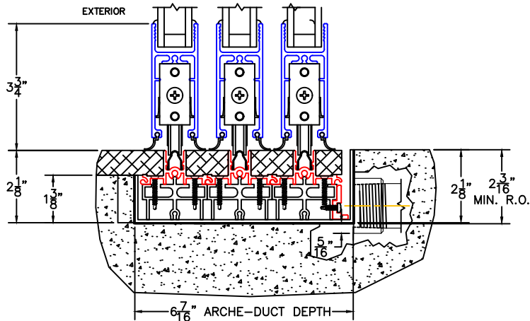
2 1" SIDE DRAIN TO INTERIOR (OPT-D1)
