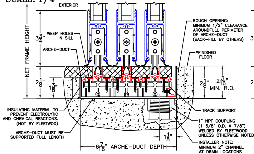
1 1" BOTTOM DRAIN TO INTERIOR (OPT-A)
