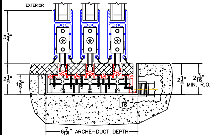
3 1/2" SIDE DRAIN TO INTERIOR (OPT-D2)
