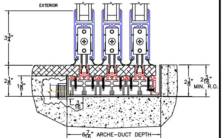
3A 1/2" SIDE DRAIN TO EXTERIOR (OPT-E2)
