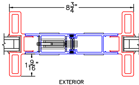
ARCHETYPE NARROW MEETING STILES WITH HP2 ADAPTERS
