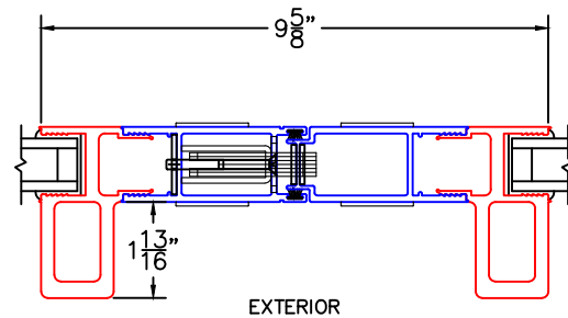
ARCHETYPE NARROW MEETING STILES WITH HP1 ADAPTERS
