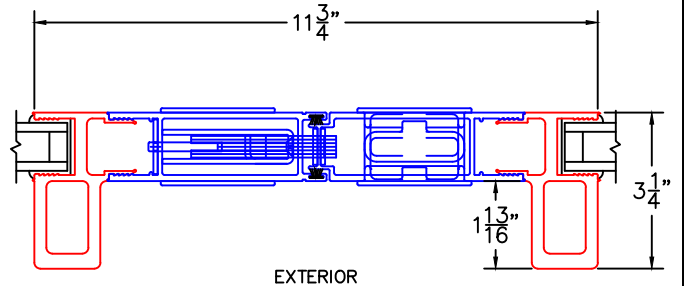
ARCHETYPE MEETING STILES WITH HP1 ADAPTERS
