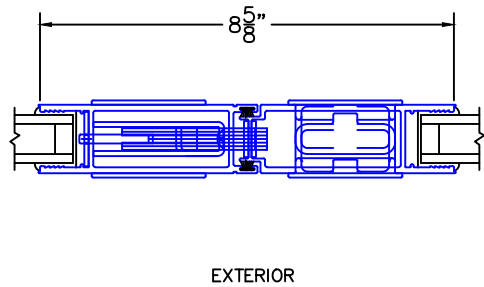
ARCHETYPE MEETING STILES
