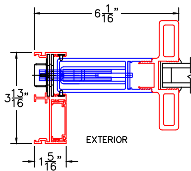
ARCHETYPE LOCK STILE WITH HP2 ADAPTER
