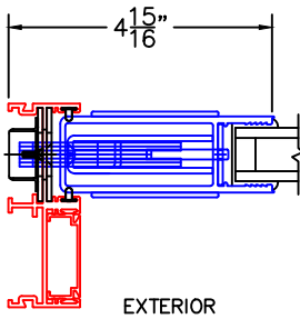
ARCHETYPE LOCK STILE
