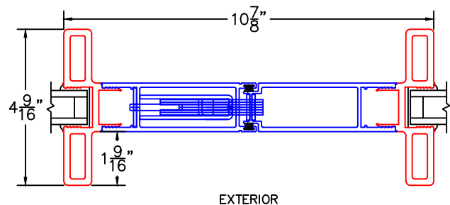
ARCHETYPE MEETING STILES WITH HP2 ADAPTERS
