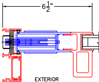
ARCHETYPE LOCK STILE WITH HP1 ADAPTER
