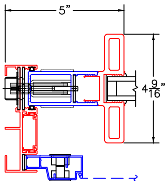
ARCHETYPE NARROW LOCK STILE WITH HP2 ADAPTER
