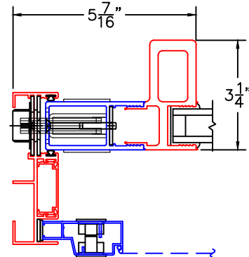
ARCHETYPE NARROW LOCK STILE WITH HP1 ADAPTER
