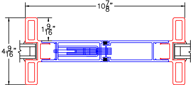
ARCHETYPE MEETING STILES WITH HP2 ADAPTERS
