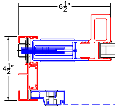
ARCHETYPE LOCK STILE WITH HP1 ADAPTER
