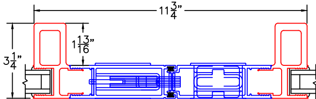
ARCHETYPE MEETING STILES WITH HP1 ADAPTERS
