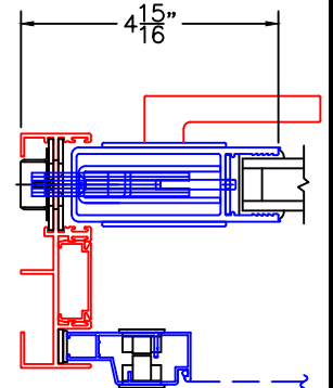
ARCHETYPE LOCK STILE WITH LEVER
