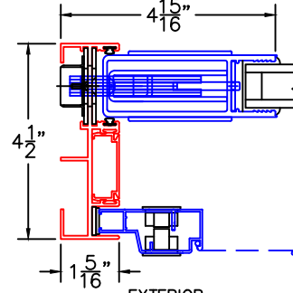
ARCHETYPE LOCK STILE
