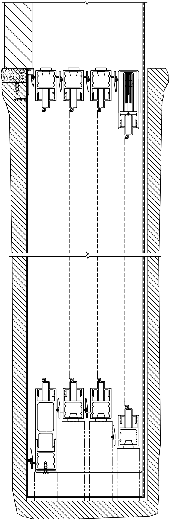
POCKET VIEW: PANELS IN OPEN POSITION
