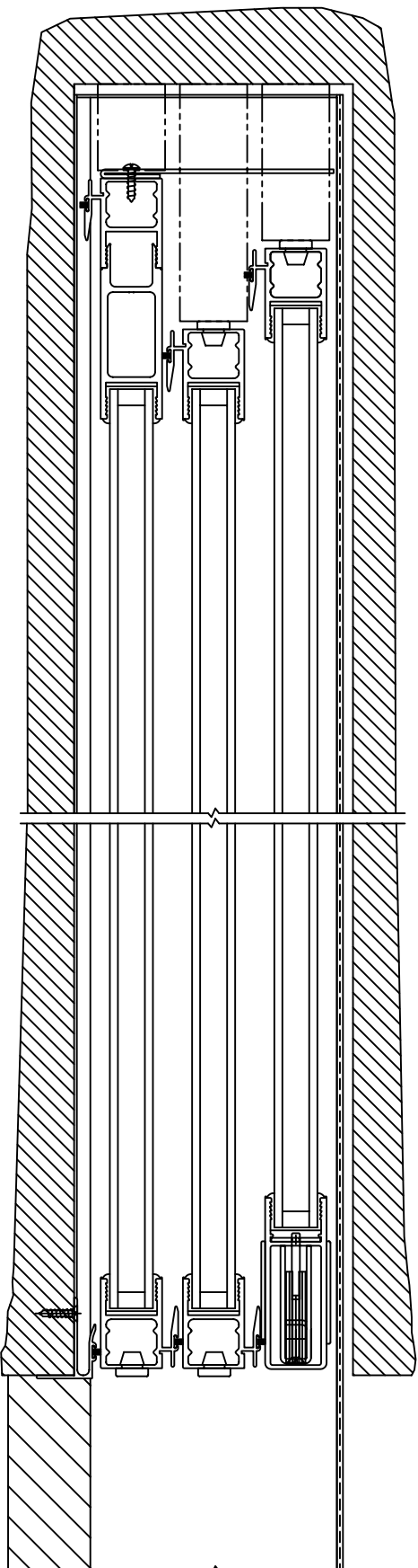
POCKET VIEW: PANELS IN OPEN POSITION
