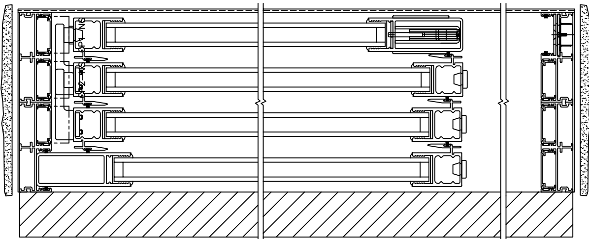
FLUSH STACK: PANELS IN OPEN POSITION
