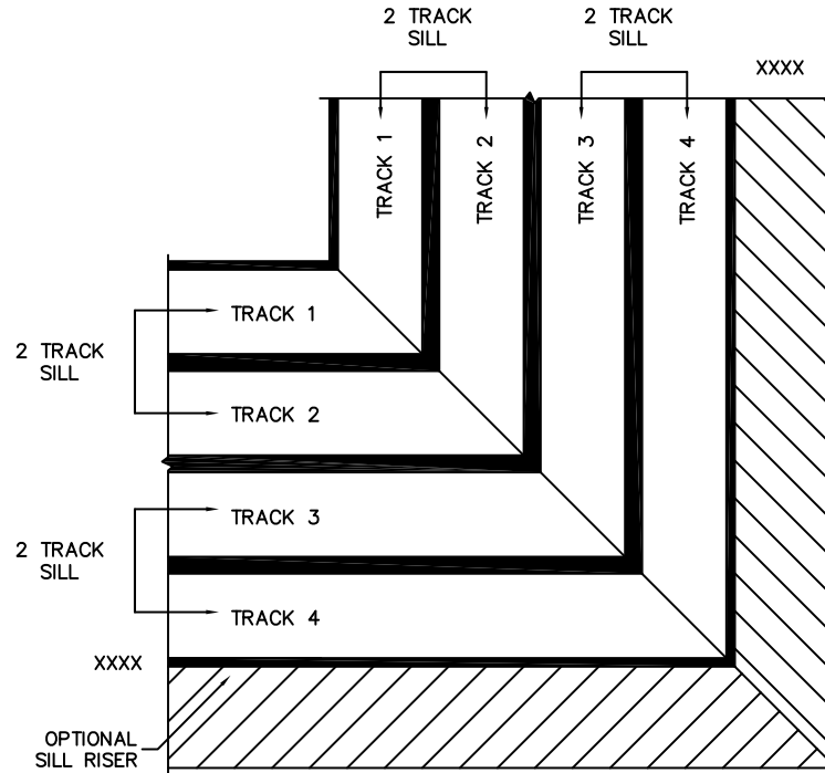
SILL TRACK MITRED CONNECTION
