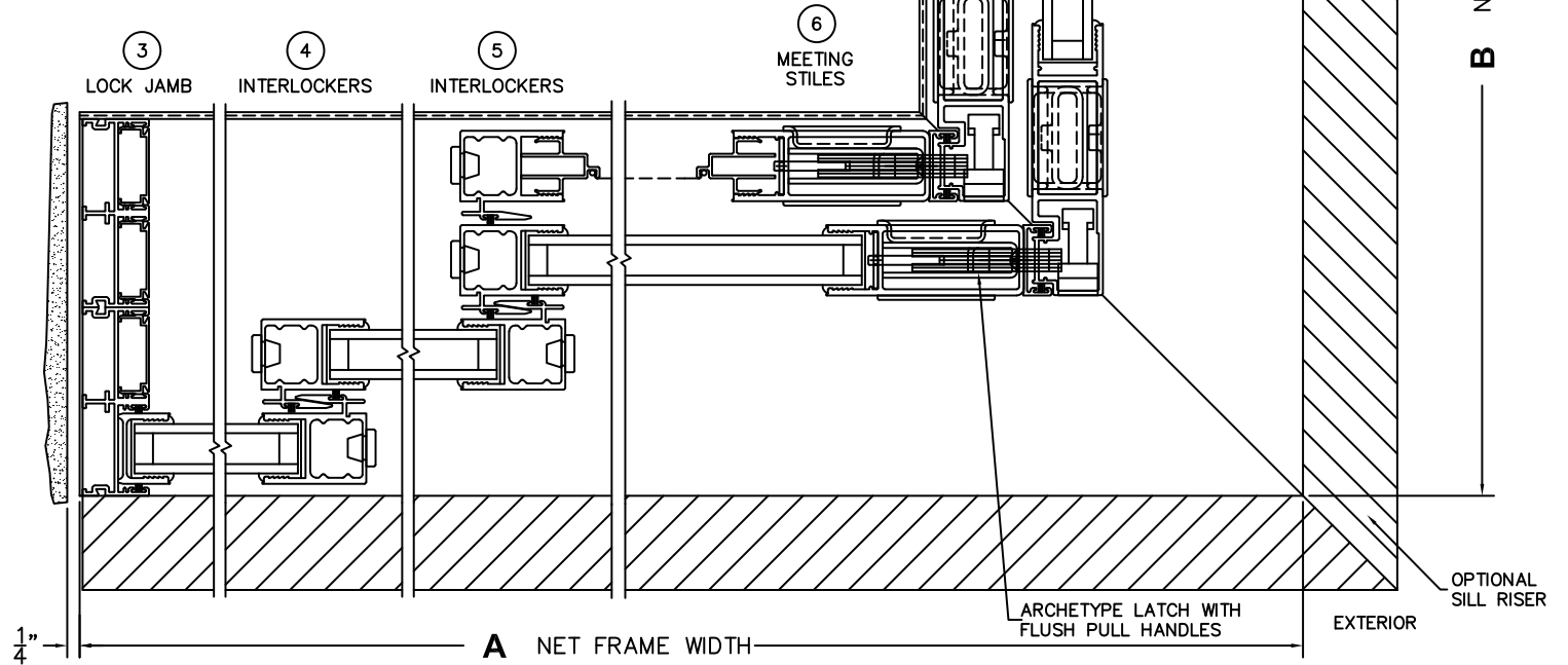
SILL TRACK MITRED CONNECTION
