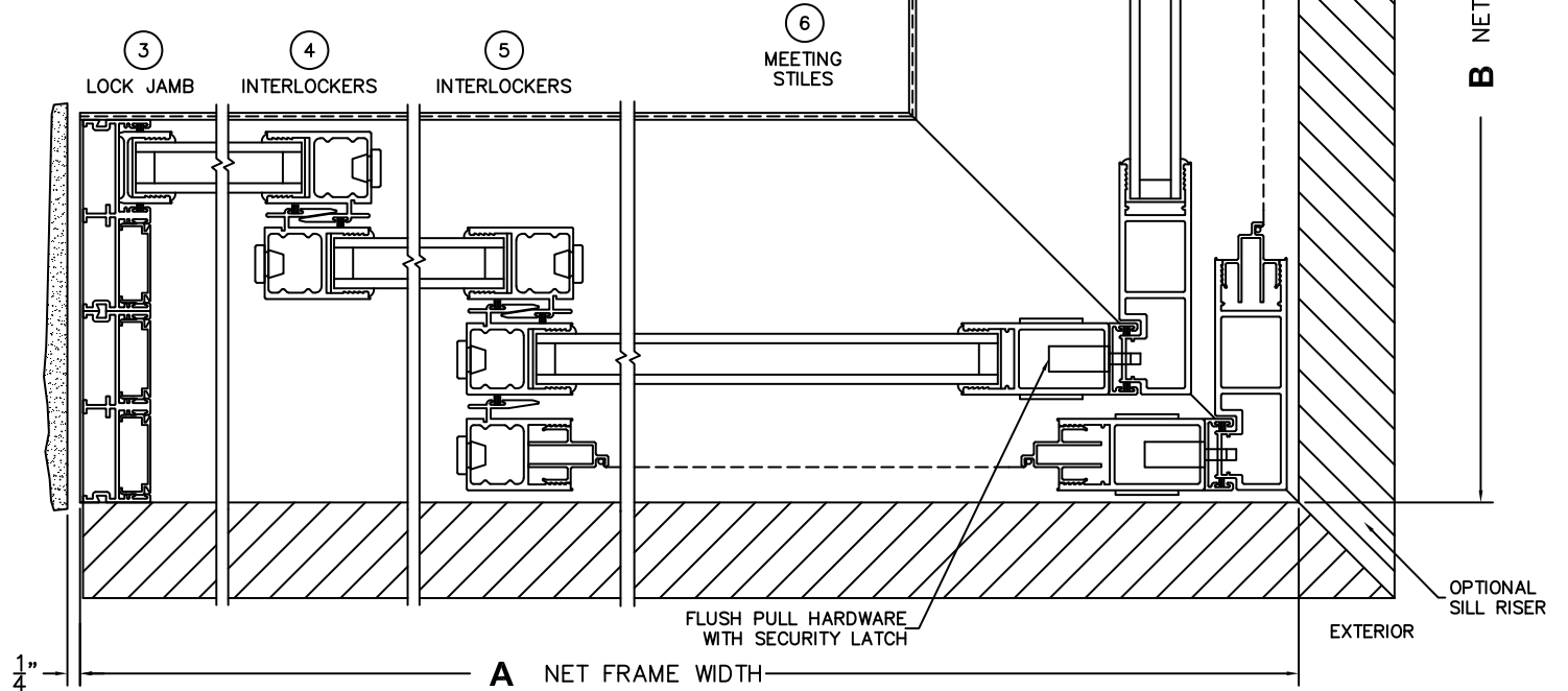
SILL TRACK MITRED CONNECTION
