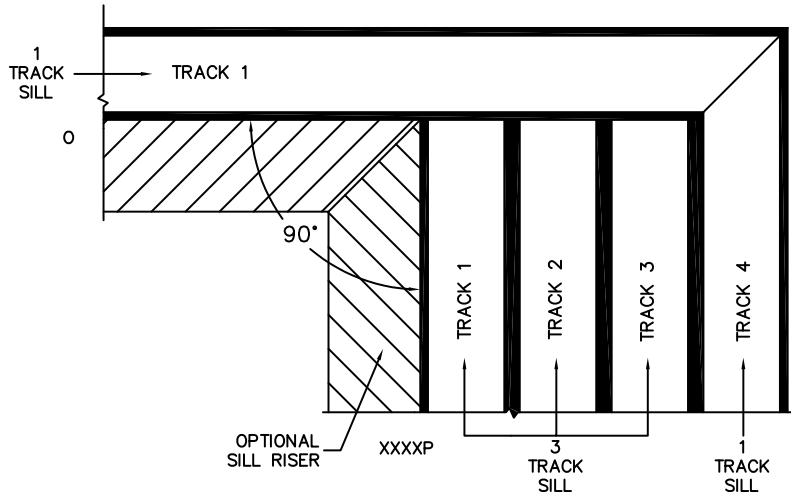
SILL TRACK MITRED CONNECTION
