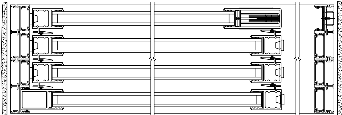
FLUSH STACK: PANELS IN OPEN POSITION
