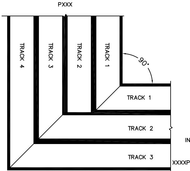
SILL TRACK MITRED CONNECTION
