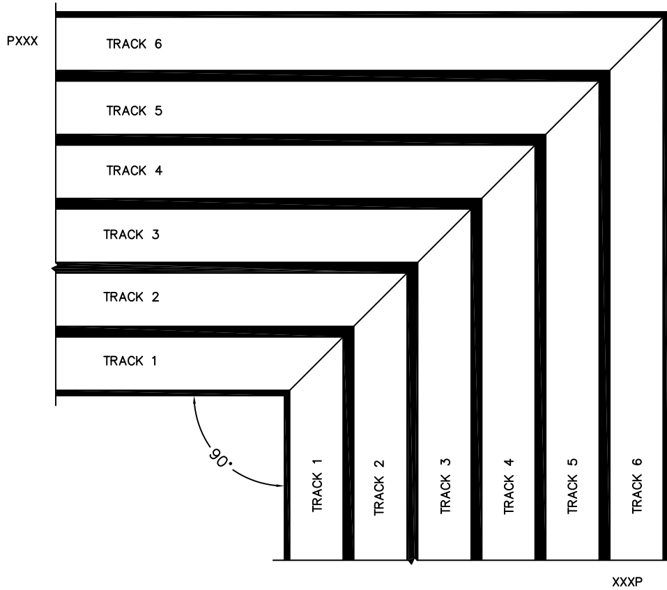
SILL TRACK MITRED CONNECTION
