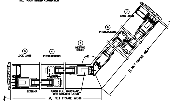
SILL TRACK MITRED CONNECTION
