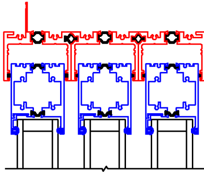
1 SERIES 4070-T HEAD
