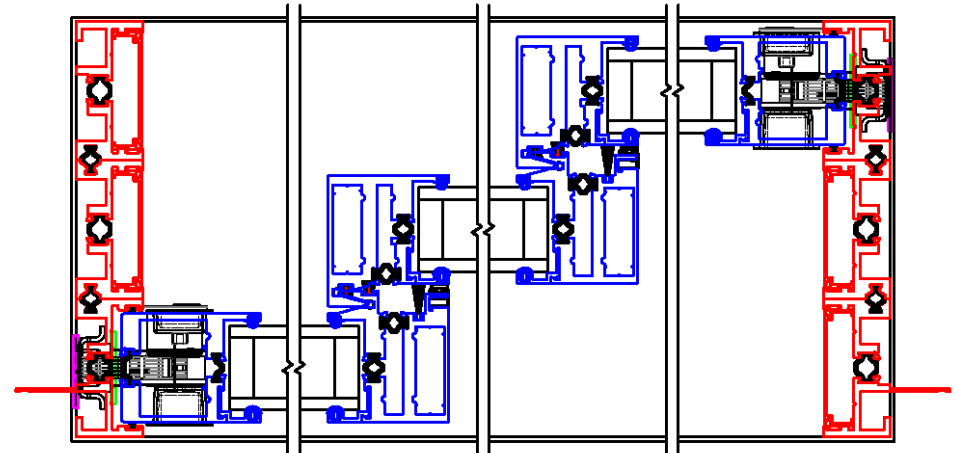
3 SERIES 4070-T PLAN VIEW
