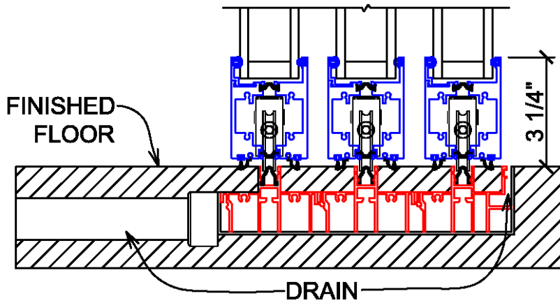
2 SERIES 4070-T SUBSILL
