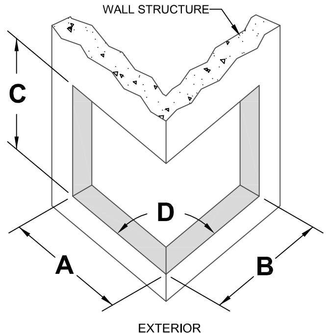
ISOMETRIC VIEW LESS THAN 90° OUTSIDE CORNER STRUCTURE
