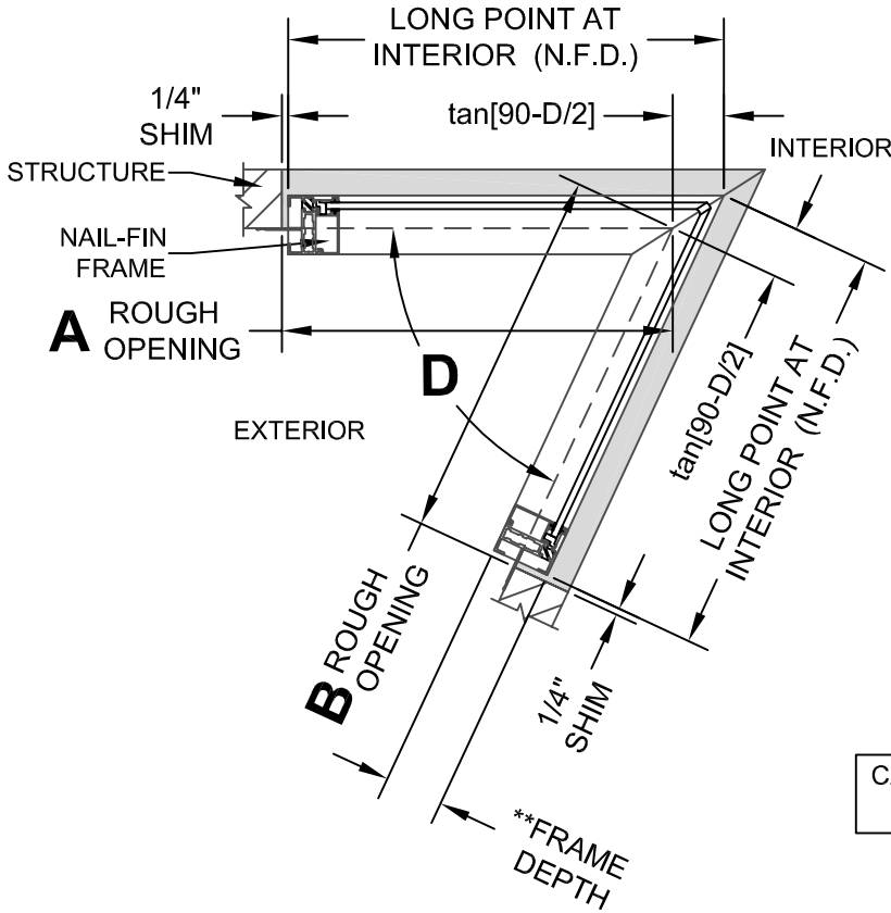
PLAN VIEW SERIES 250-T SHOWN
