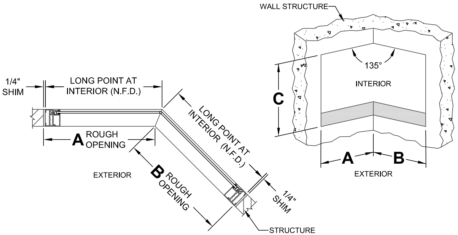
PLAN VIEW SERIES 250-T SHOWN
