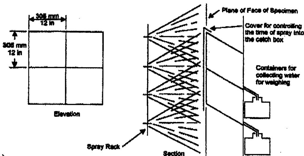
FIG. 2 Catch Box for Calibrating Water-Spray System
