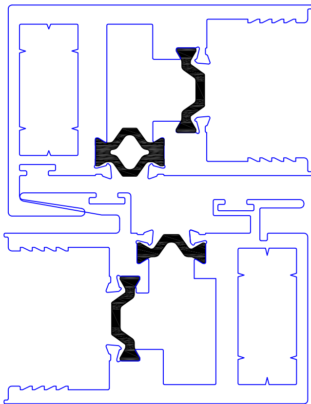
STANDARD THERMAL INTERLOCKERS
